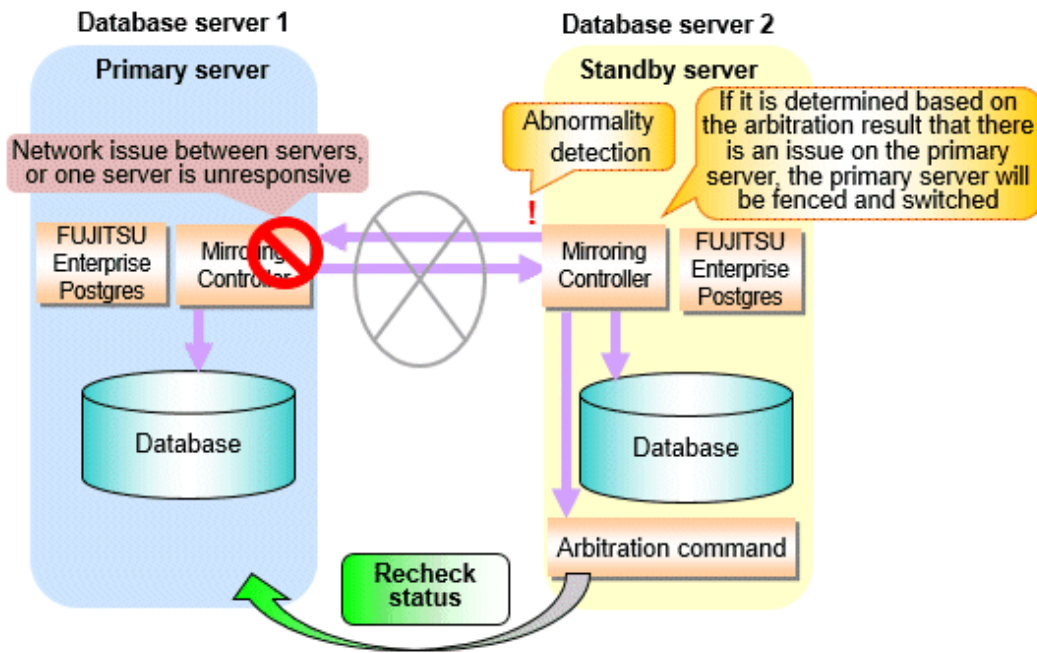
Figure 1.4 Database degradation using the arbitration command
