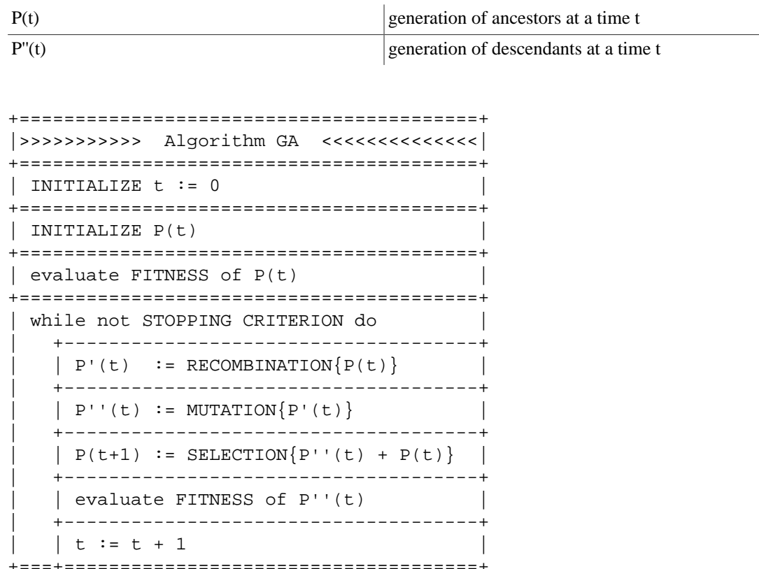
Figure 59.1. Structured Diagram of a Genetic Algorithm
