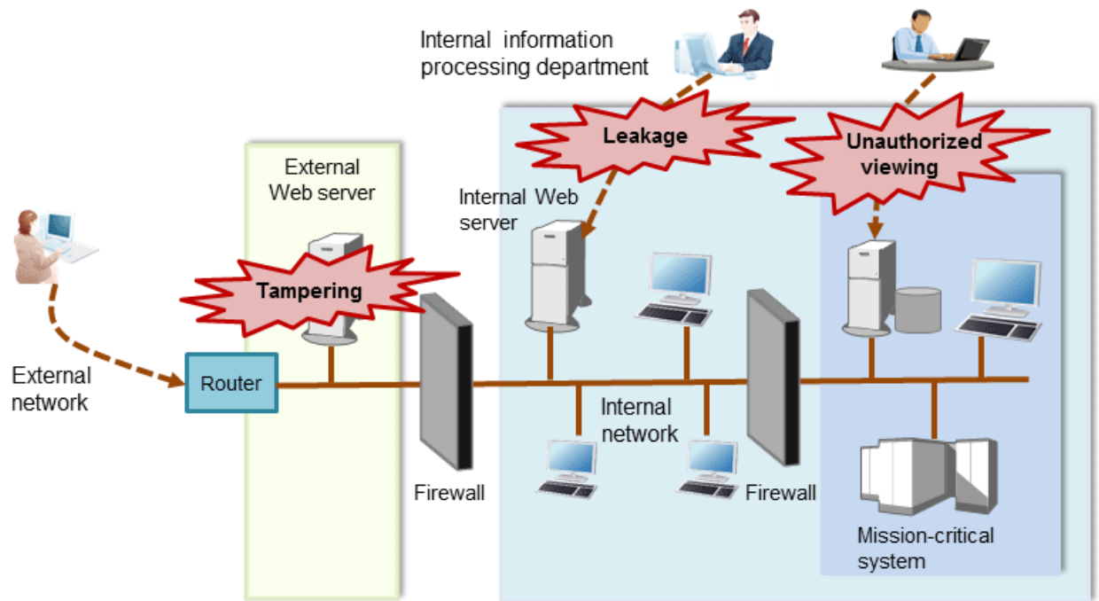
Figure 1.1 Security threats
