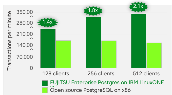
TPC-C throughput: FUJITSU Enterprise Postgres on IBM LinuxONE III vs Open source PostgreSQL on x86
